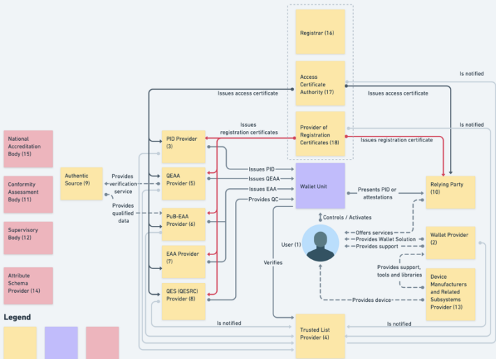
ARF – Architecture Reference Framework
